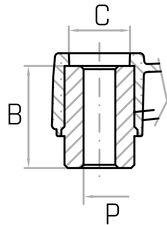
Mod. MHP-PGR
